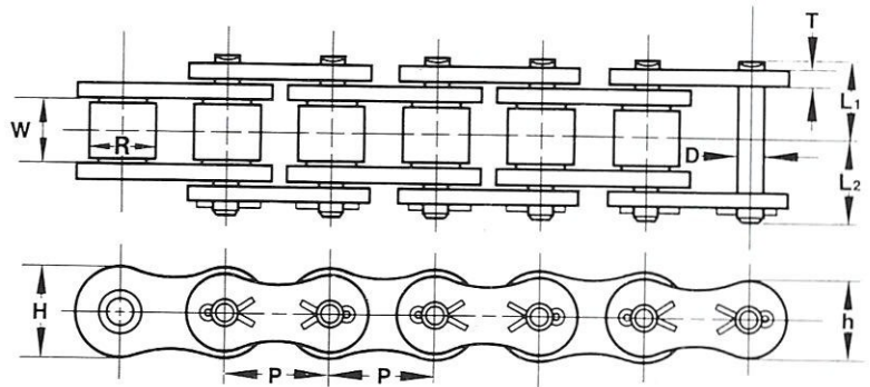
COTTERED TYPE
