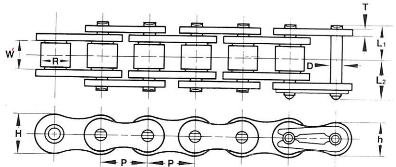
RIVETED TYPE
